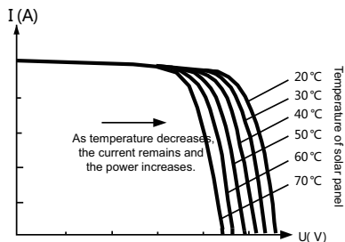
Fig. 2-3 Relationship between output characteristic of battery panel and temperature
