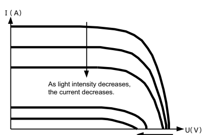
Fig. 2-2 Relationship between output characteristic of battery panel and light intensity
